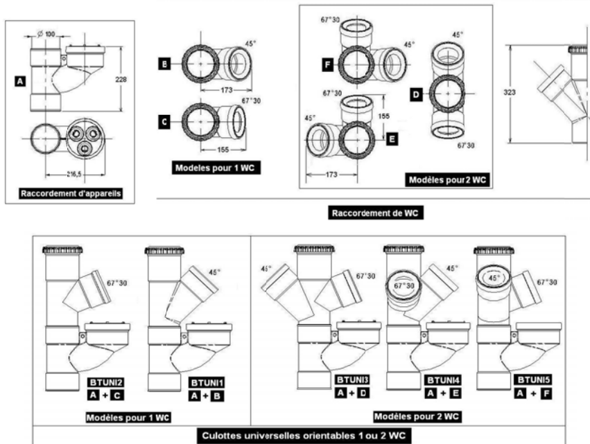
Figure 2 - Culottes universelles orientables
